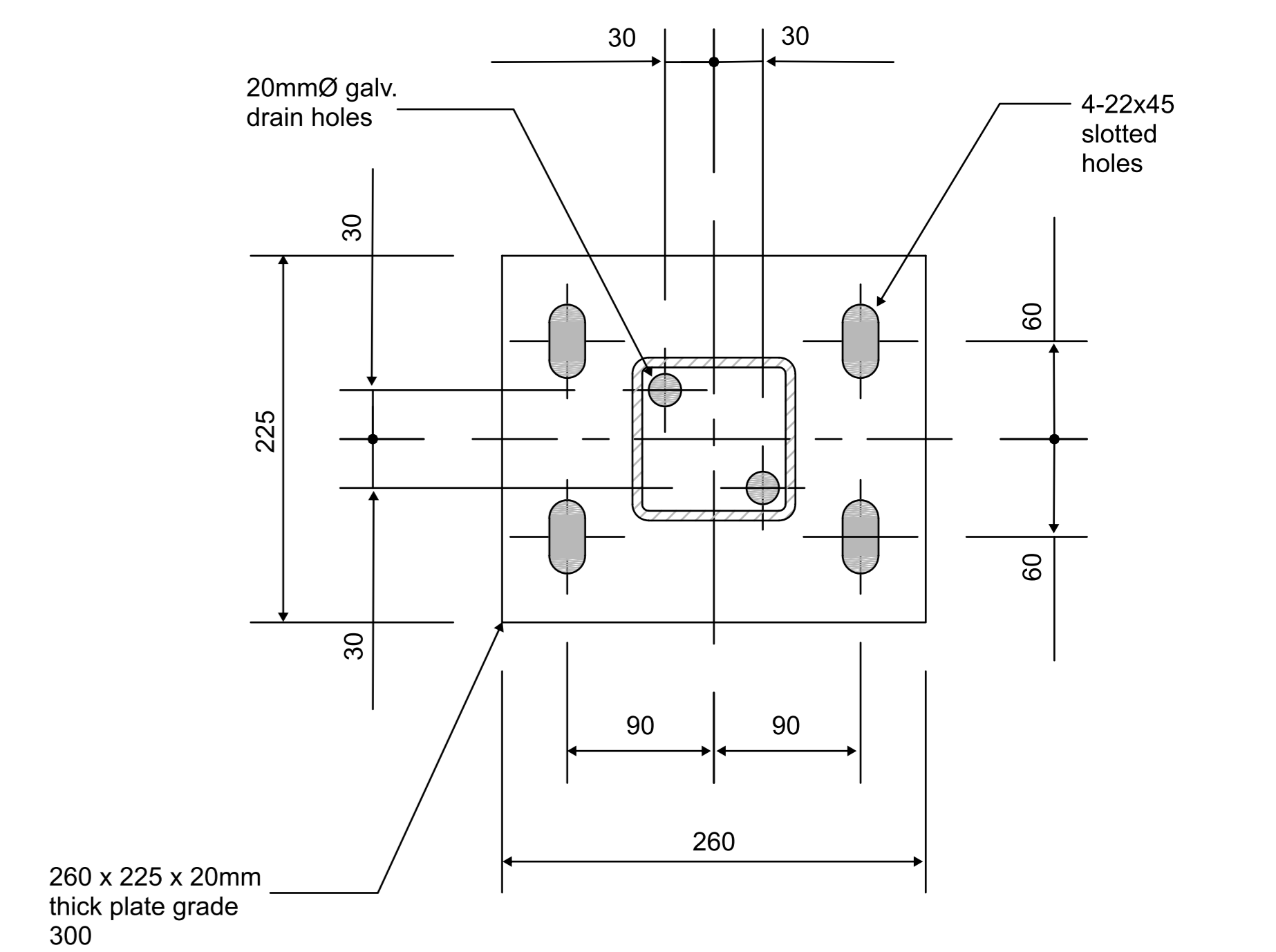
BASE PLATE
