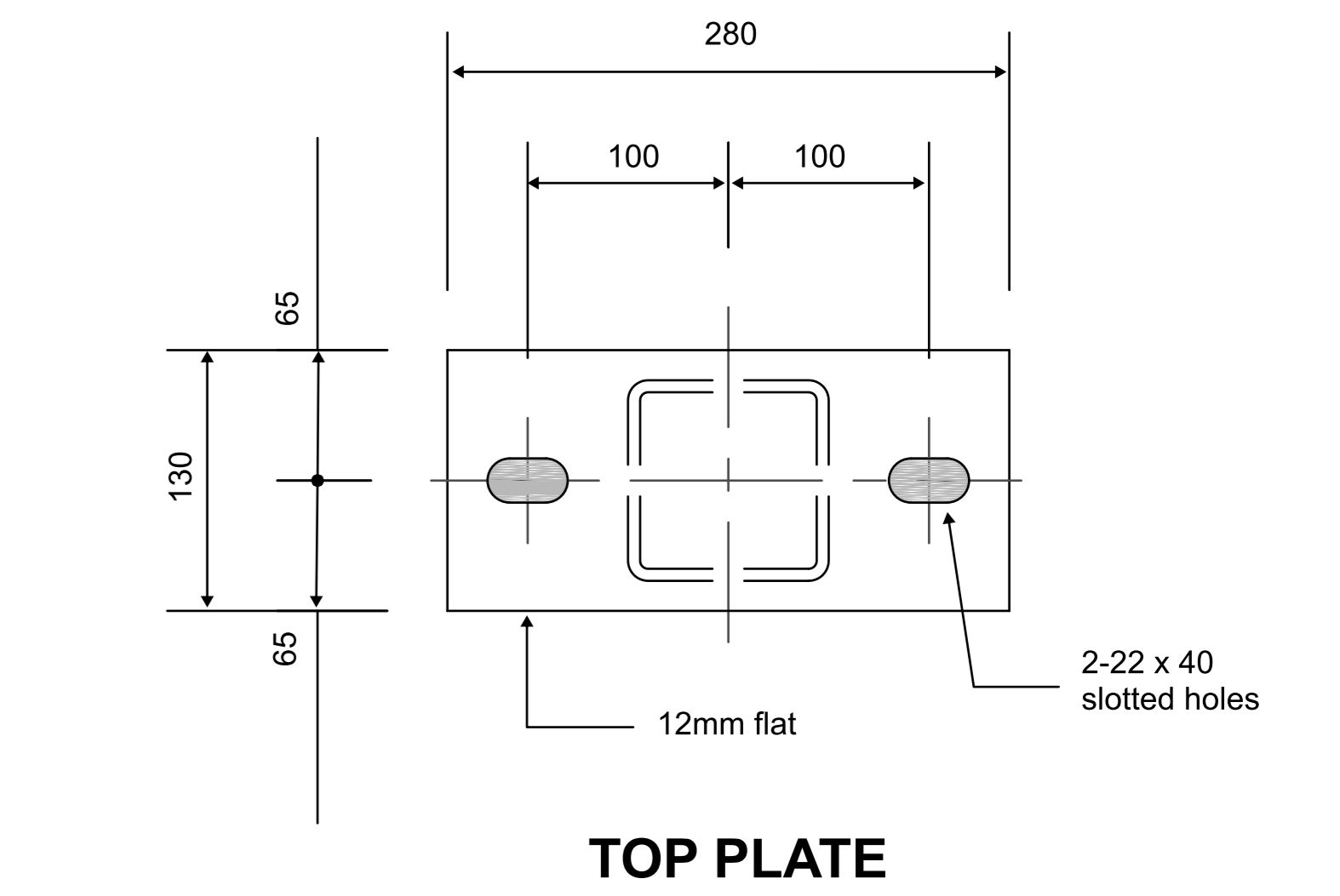
TOP PLATE
