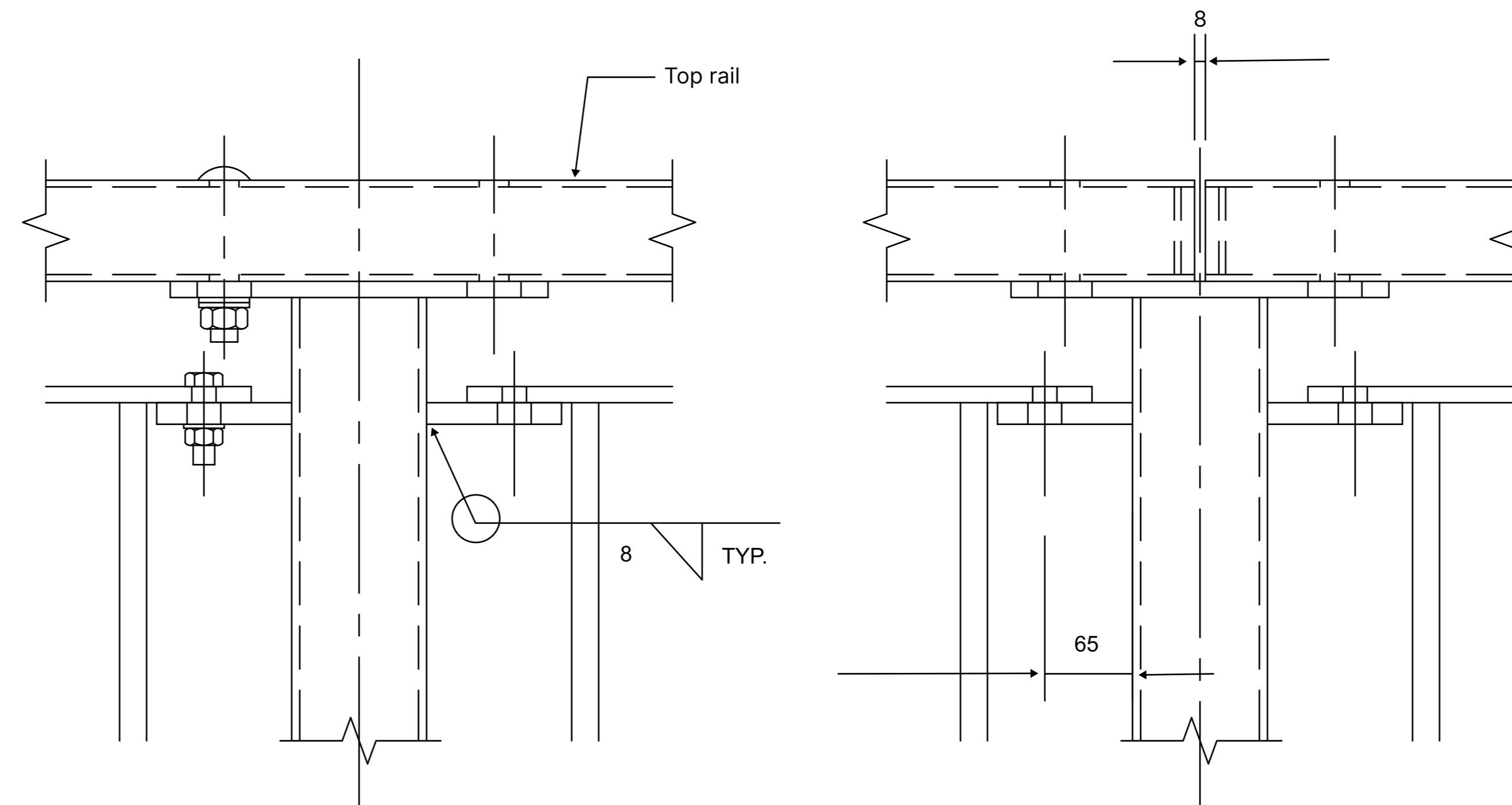
TOP RAIL CONTINUOUS
