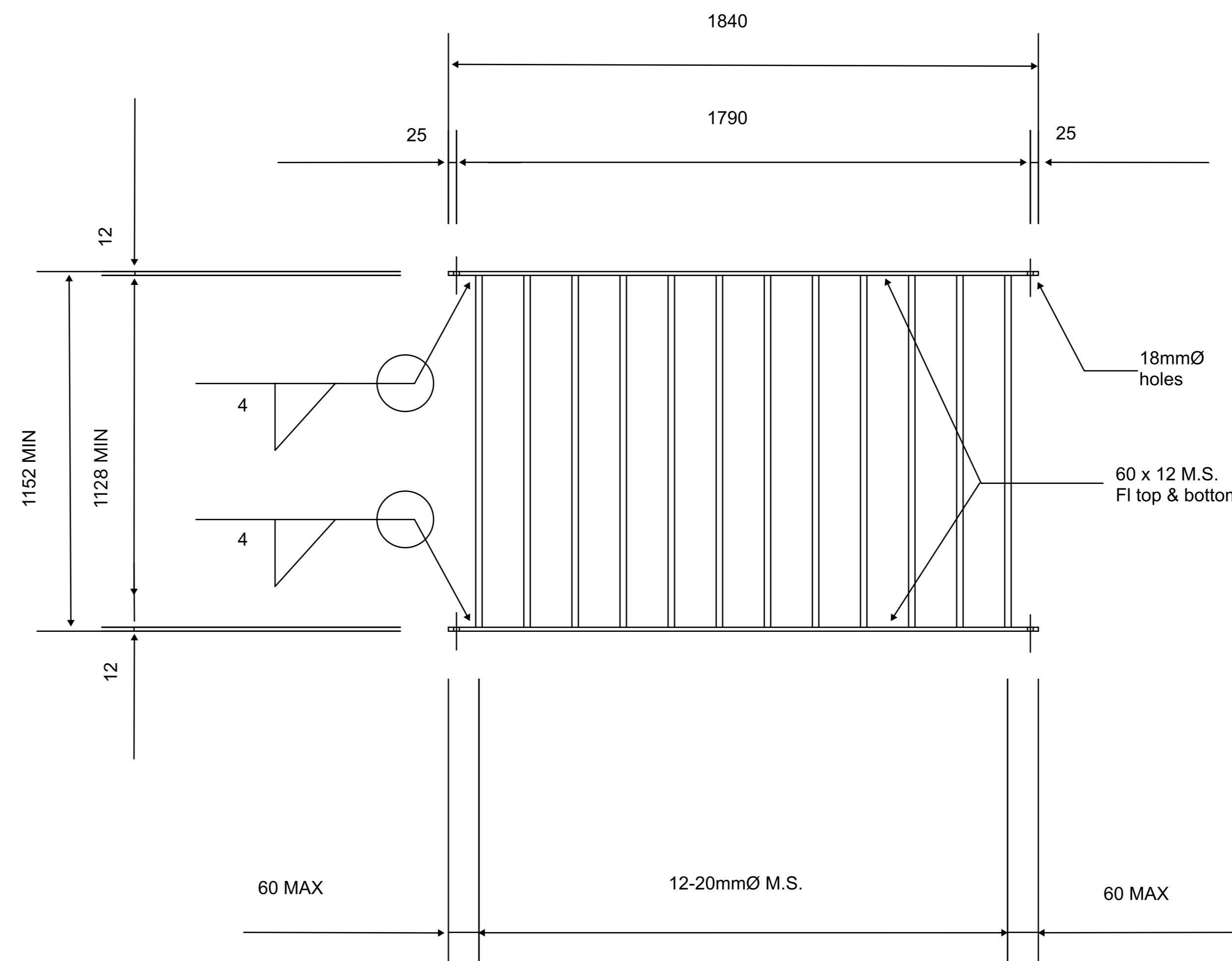
PANEL DETAIL
